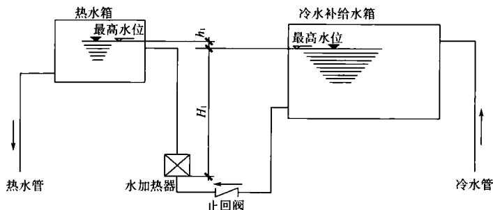
图8 热水箱与冷水补水箱布置
